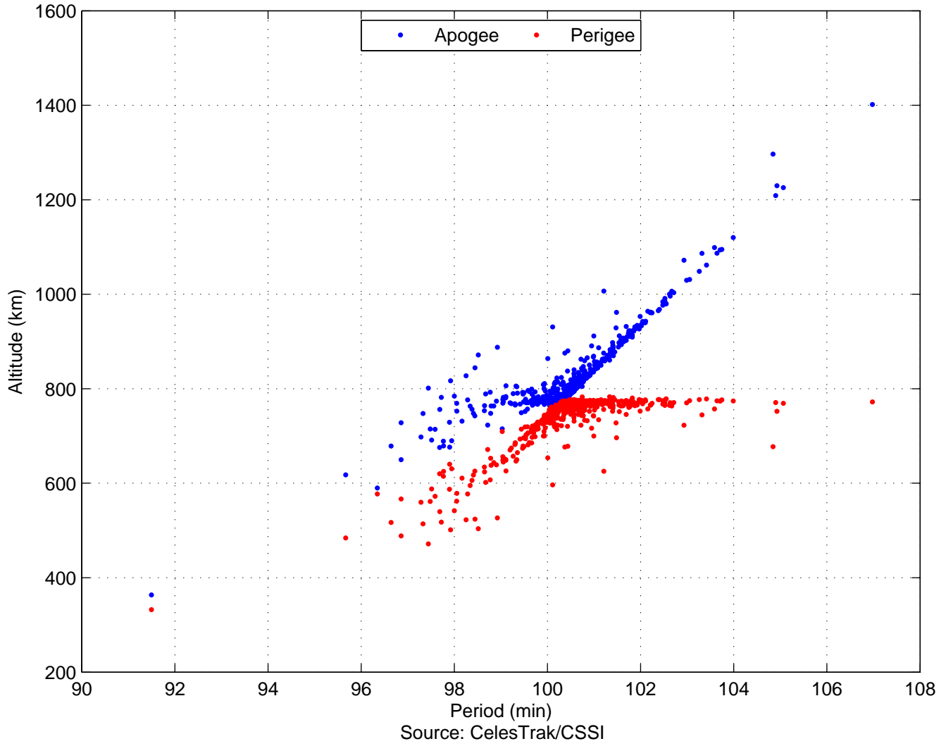
Gabbard Plot of Iridium 33 Debris (477 pieces)
