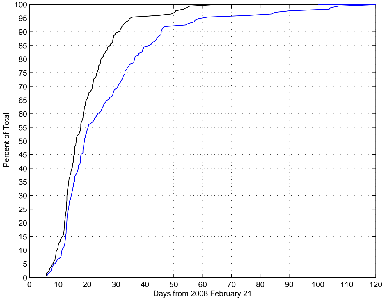
Lifetime Plot of USA 193 (2006–057) Debris (173 pieces)
